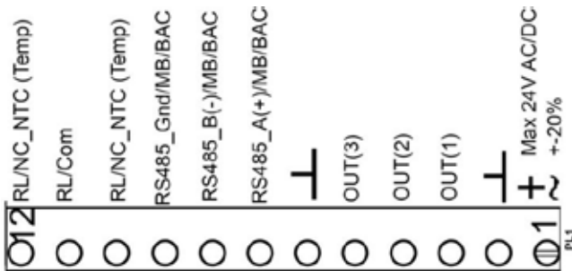
Figur 3: Kopplingsplint
